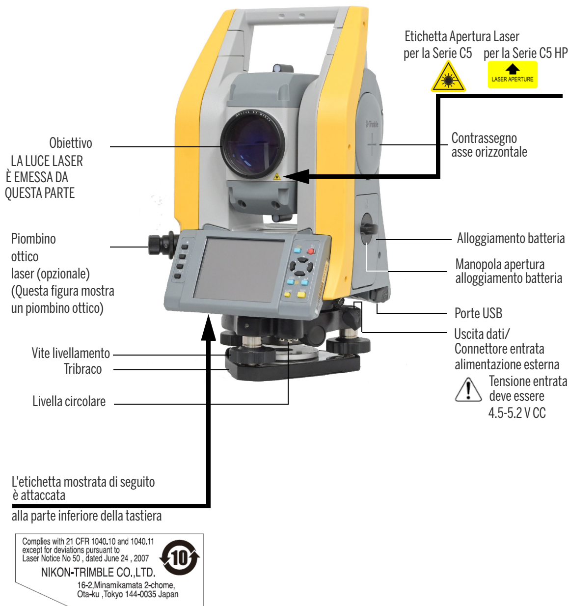
Figura 1.2 Trimble C5 Series total station – Faccia-2
